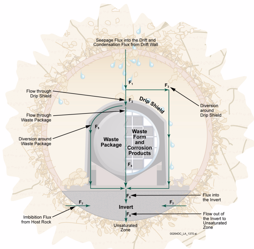
Figure 6-1. Potential Flow Pathways in the Engineered Barrier System (SAR Figure 2.3.7-8; DOE, 2008ab)
